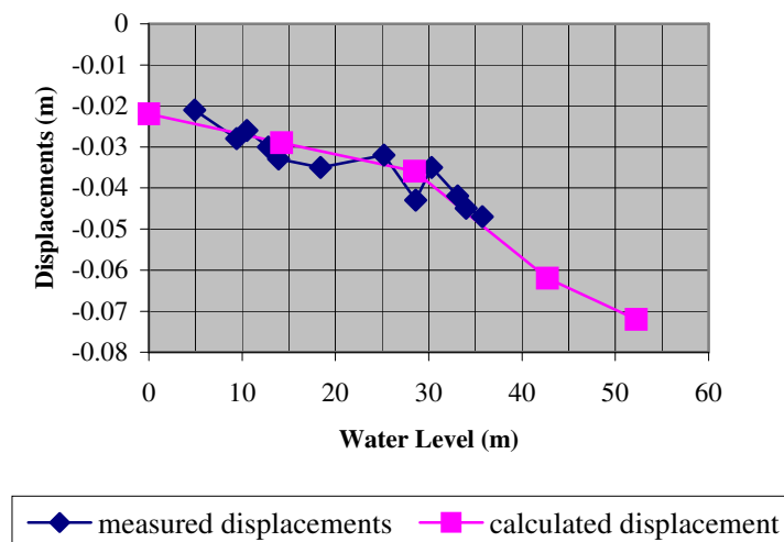
Fig.7. Calculated and measured displacements at the crest of the East Dam.
